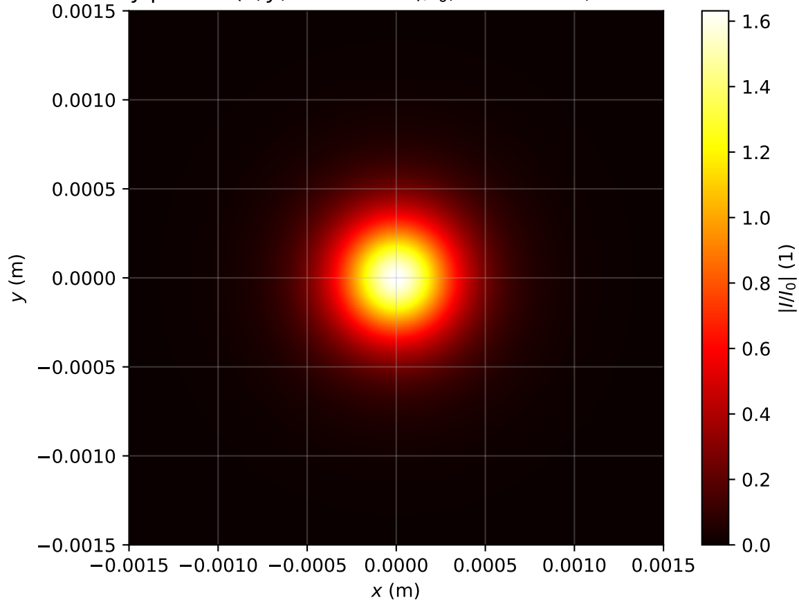
Intensity profile I(x, y, z = 1.990m)/I_0 , \text{Pin}=0.9\text{Pcr} , artificial time
